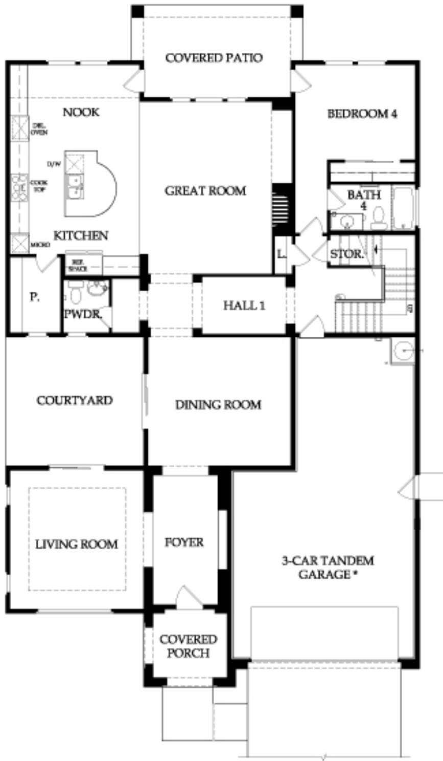
ELEVATION 'A' First Floor
