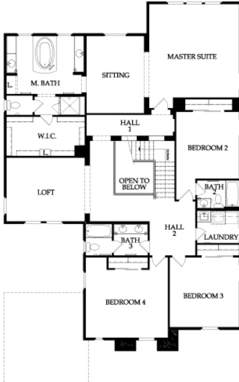
ELEVATION 'A' Second Floor
